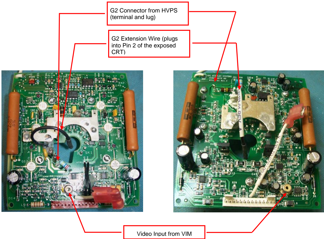
Earlier Design 03-270338-01P/02P/03P 03-270339-01P
