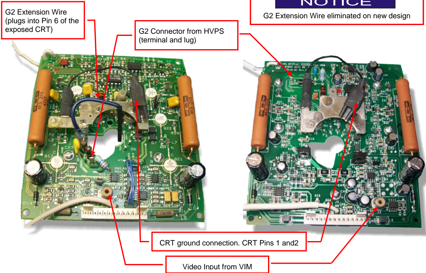
Earlier Design 03-270339-02P/03-270339-03P
